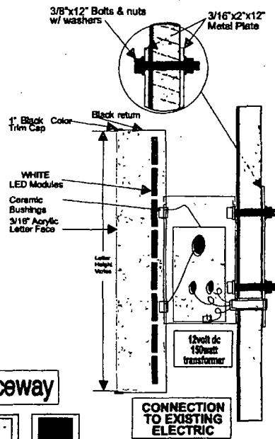
CHANNEL LETTER DETAIL NOT SCALE
