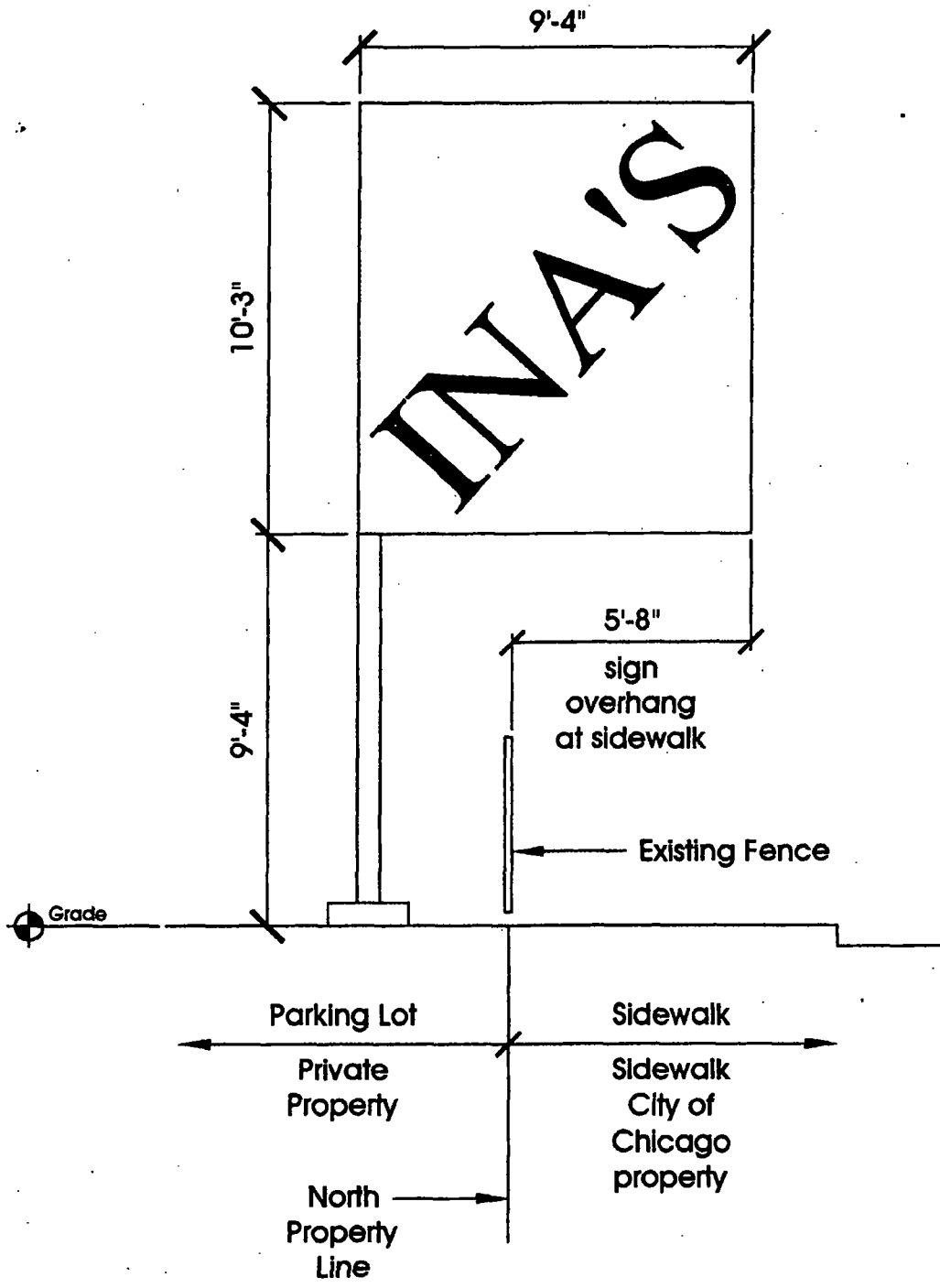
Elevation: Existing Sign
