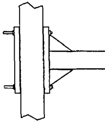
DETAIL OF BEAM MOUNT 3" STEEL TUBE/GUSSETS WELDED TO .5" STEEL PLATE/BOLTED TO BACKING PLATE WITH 5" GALV. BOLTS
