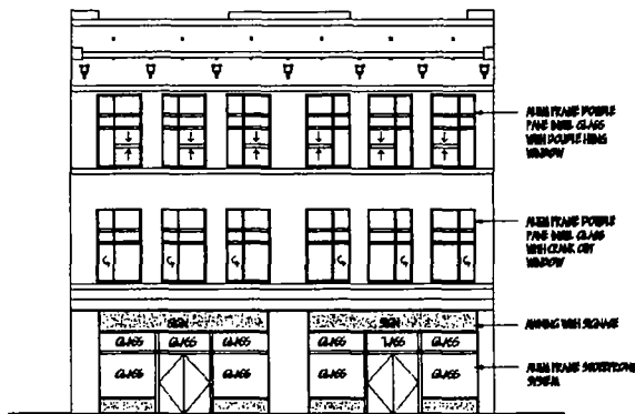
1 NORTH ELEVATION 5/16" = 1'-0"
