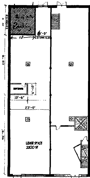
1 FIRST FLOOR PLAN 3/16" = 1'-0"
