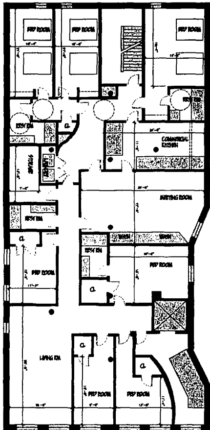
3 THIRD FLOOR PLAN
