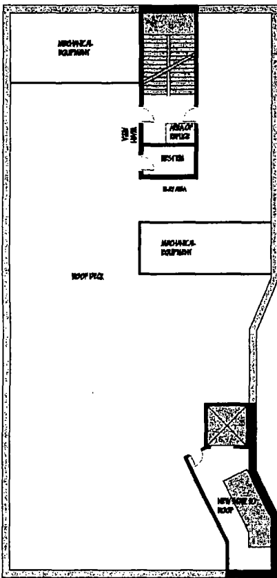
4 ROOF PLAN 3/16" = 1'-0"
