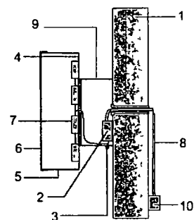
LED Channel Letter Side View
