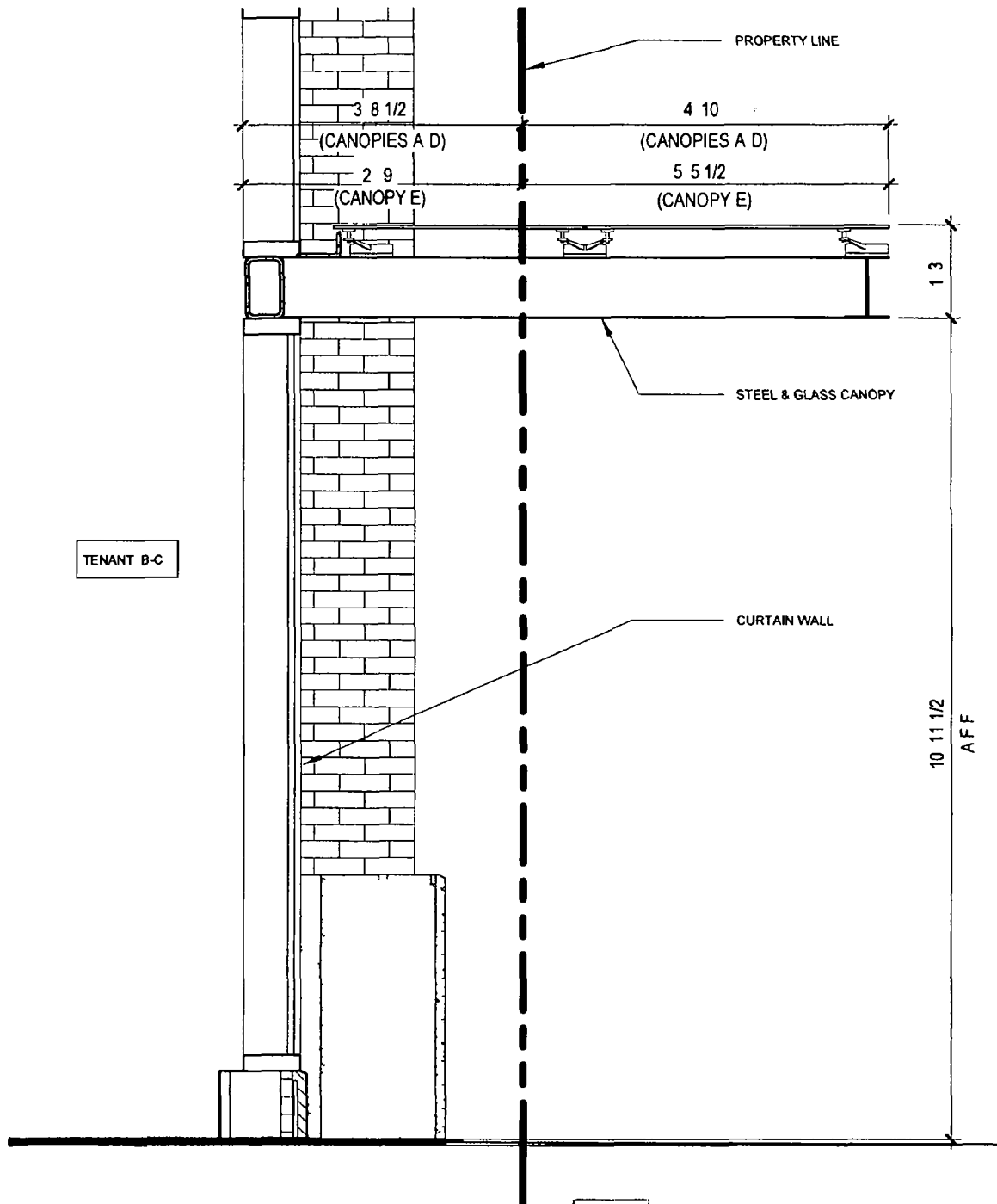
1 TYPICAL AT CANOPIES A-E C-SK03 1/2" = 1'-0" A8 01A 0 1 2
