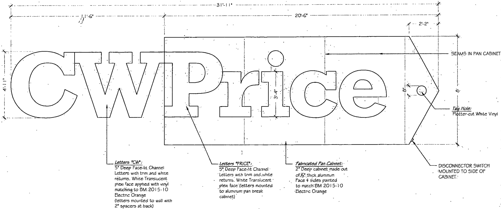
1 SIGN TYPE - C (60" tall) Face-Lit Channel Letters & Cabinet
