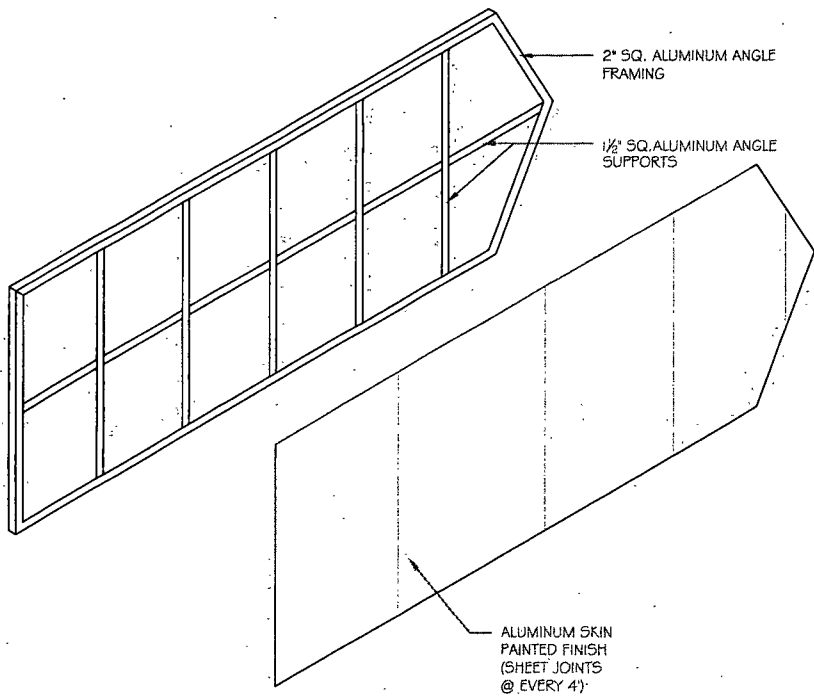
1 ISOMETRIC VIEW FRAMING & SKIN - CABINET
