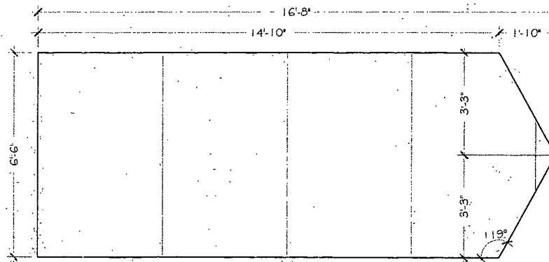
1 ELEVATION - CABINET SIGN TYPE - 'A' & TYPE - 'B'
