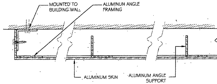
2 PART SECTION THRU CABINET
