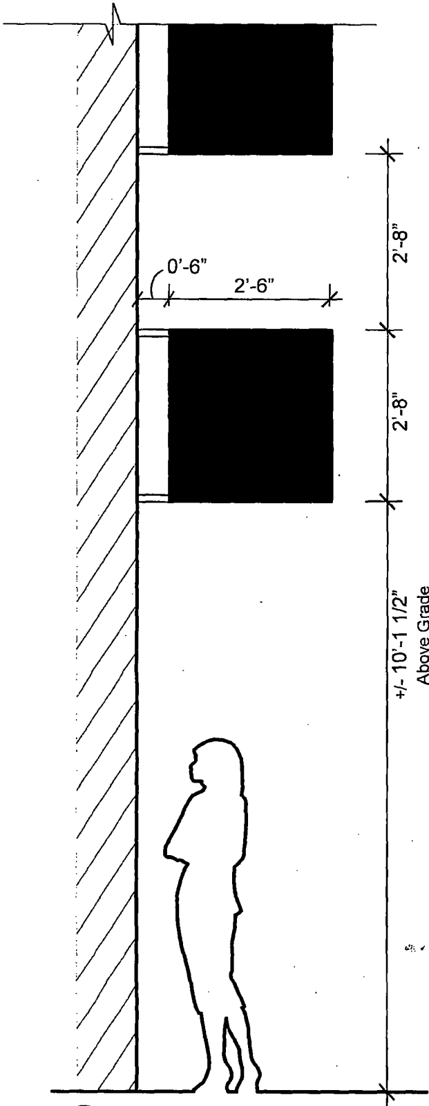
1 Blade Sign 1 Street Elevation 1/2" = 1'0"
