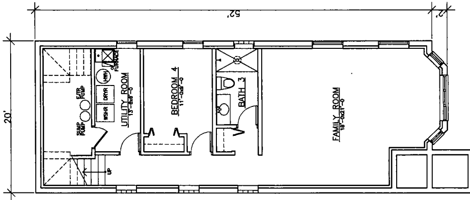
BASEMENT PLAN
