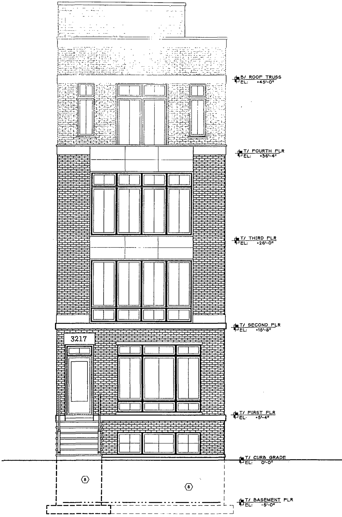
4 FRONT ELEVATION
