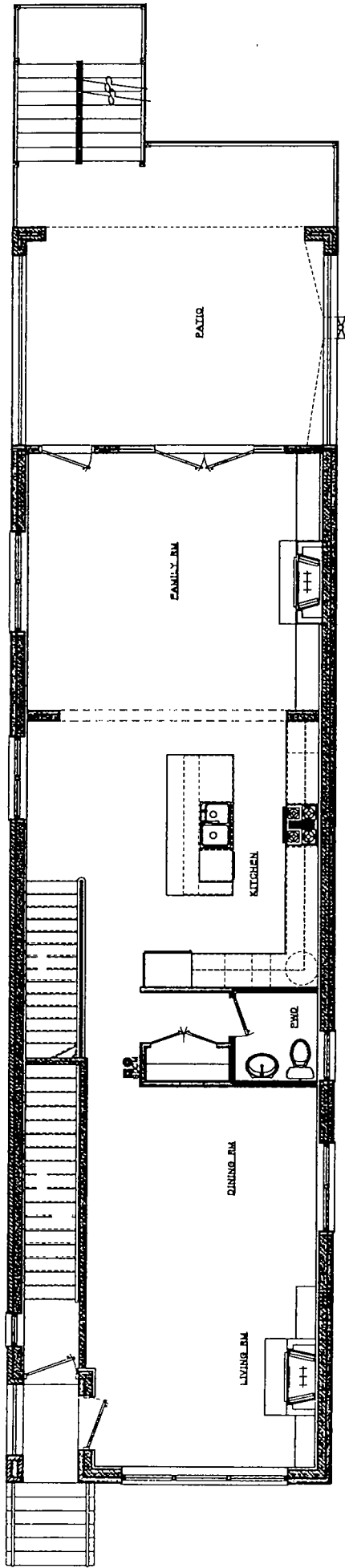
2 FIRST FLOOR PLAN
