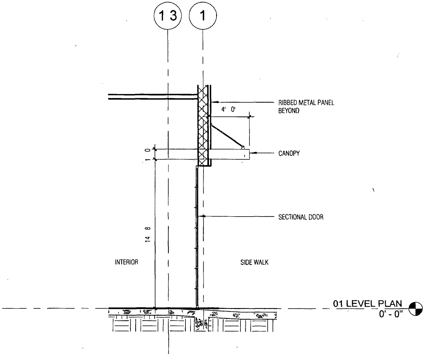
SECTION AT DRIVEWAY CANOPY
