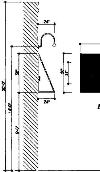
SIDE VIEW 1/4" = 1'-0"
