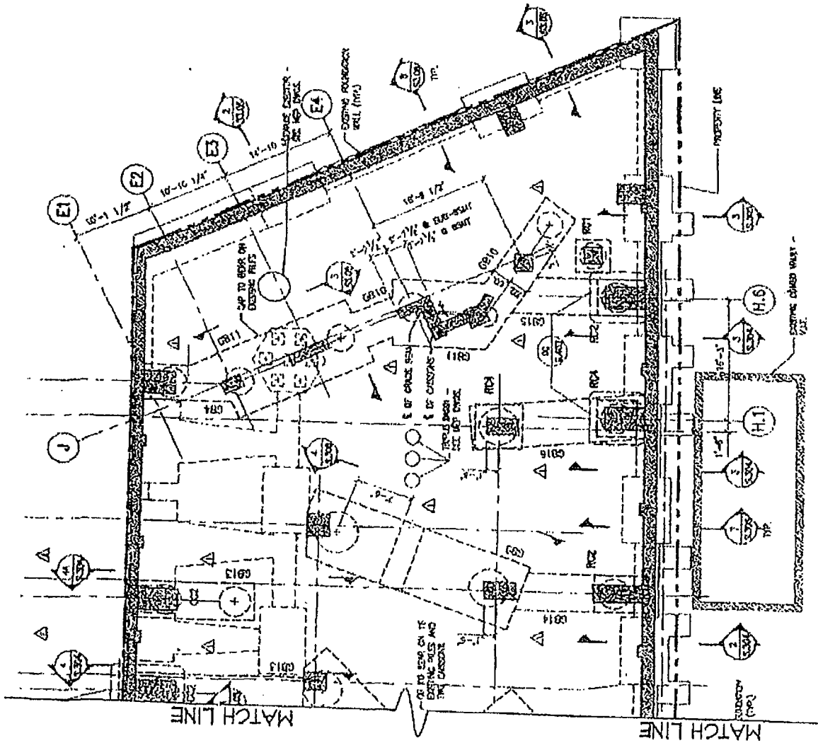
PILECAPS BELOW SUB-BASEMENT (EAST) SCALE: 1/16" = 1'-0"
