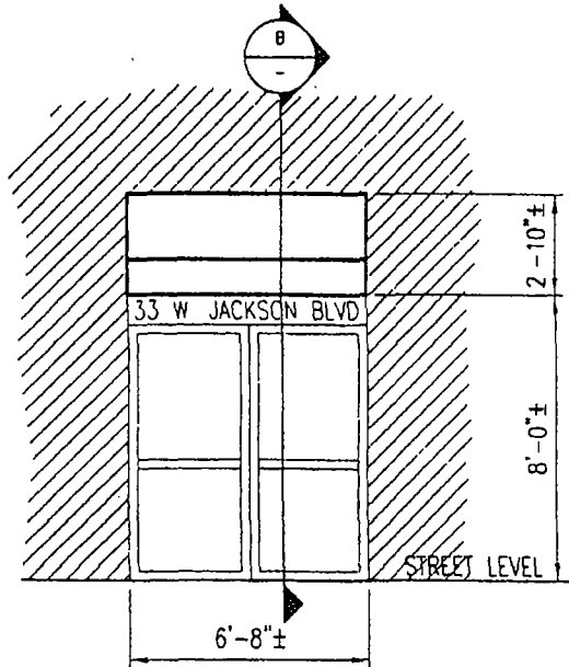
ELEVATION LOOKING SOUTH AT BUILDING A - NTS
