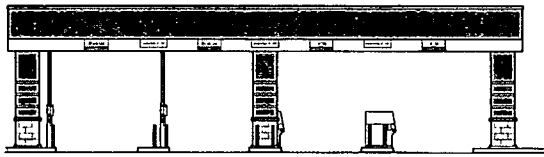
North Elevation Scale: 3/16"=1'-0"
