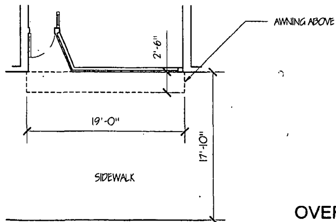
1 AWNING PLAN 1/8" = 1'-0"
