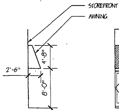
2 AWNING SECTION 1/8" = 1'-0"
