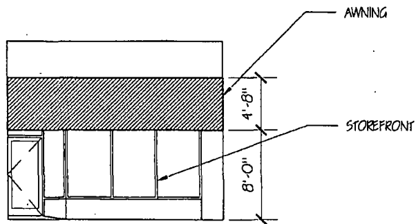
2 AWNING ELEVATION 1/8" = 1'-0"
