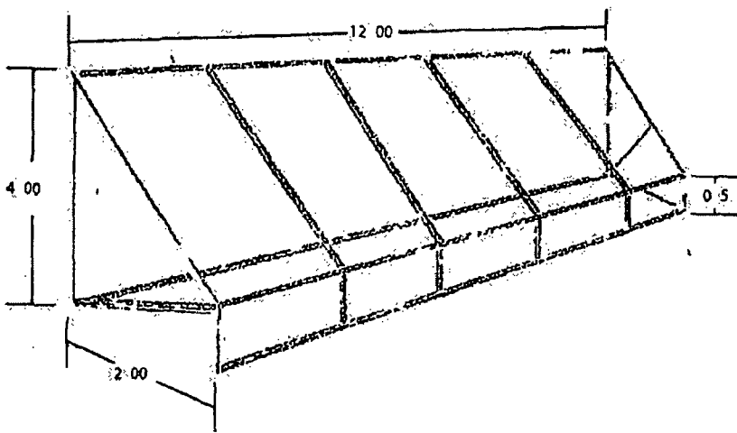
Awning structure SIDE VIEW
