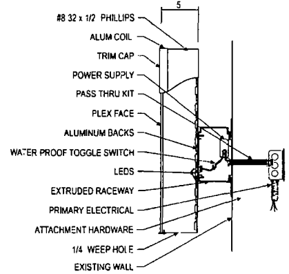
SECTION DETAIL @ CHANNEL LETTERS SCALE 1" = 1'-0"
