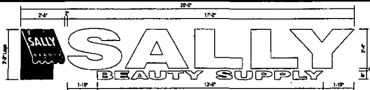
BB-300-AM (EQ.D EQ. FL) LED ILLUMINATED WHITE CHANNEL LETTERSET (REMOTE) SIGN #1 QTY 1 SCALE 3/8"=1'-0"
