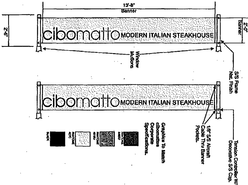
(2) D/E Non-Illuminated Banner Display 3/8" = 1'
