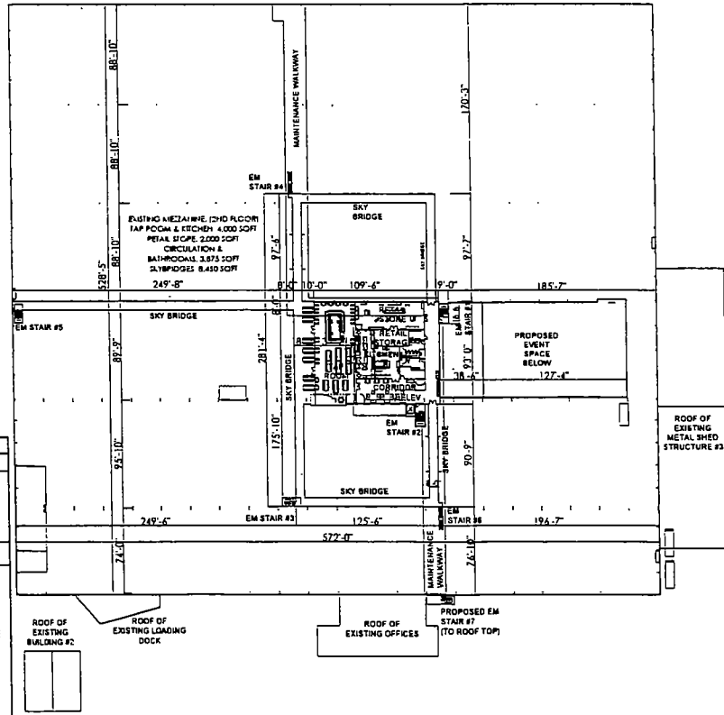
PROPOSED OVERALL SECOND FLOOR PLAN
