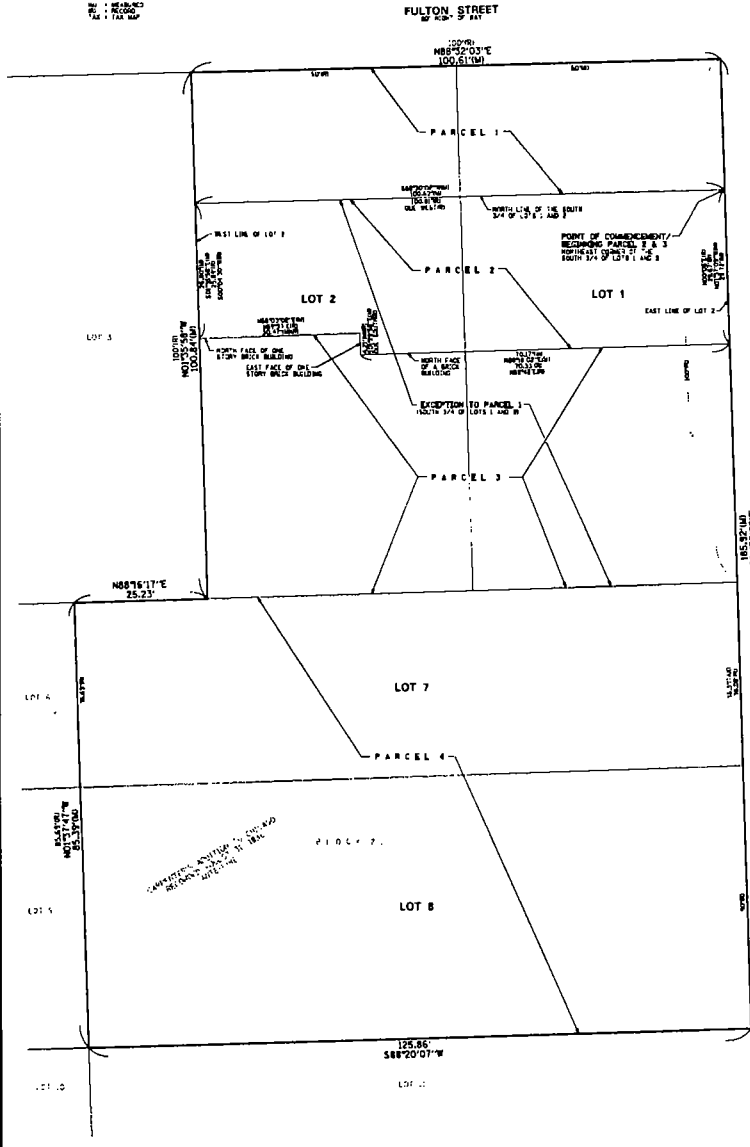
EXISTING BOUNDARY INFORMATION SCALE: 1" = 40'
