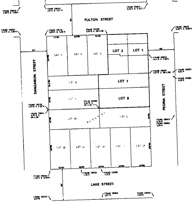
DETAIL OF FOUND MONUMENTATION SCALE: 1" = 40'
