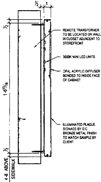
PLAQUE SIGNAGE DETAIL 10
