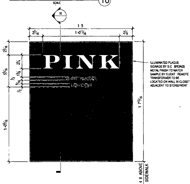
PLAQUE SIGNAGE DETAIL 8
