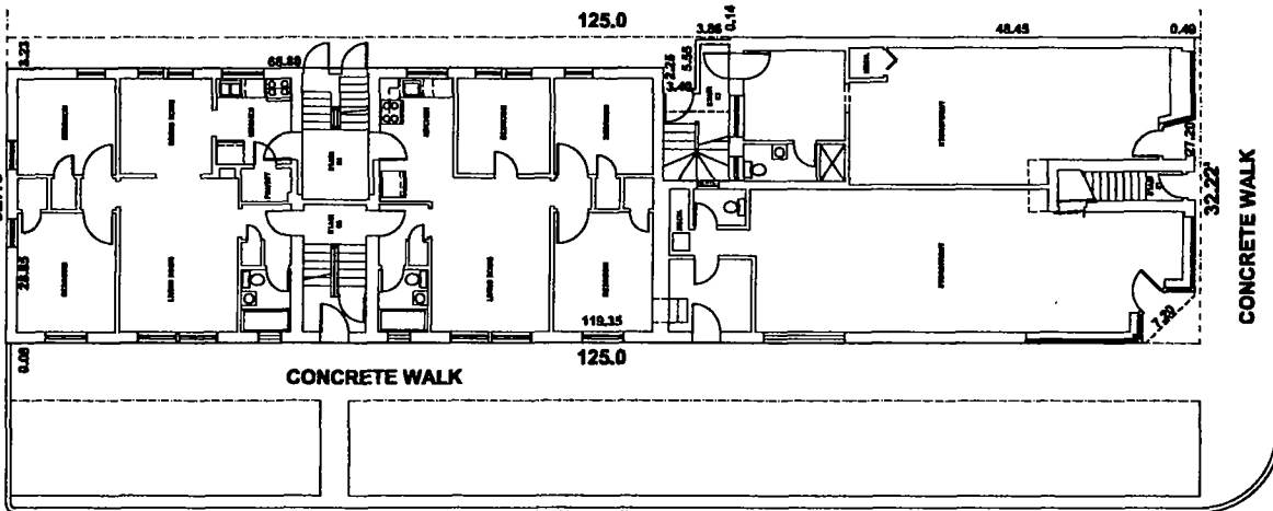
1 EXISTING FIRST FLOOR & SITE PLAN SCALE 3/8"=1'-0"
