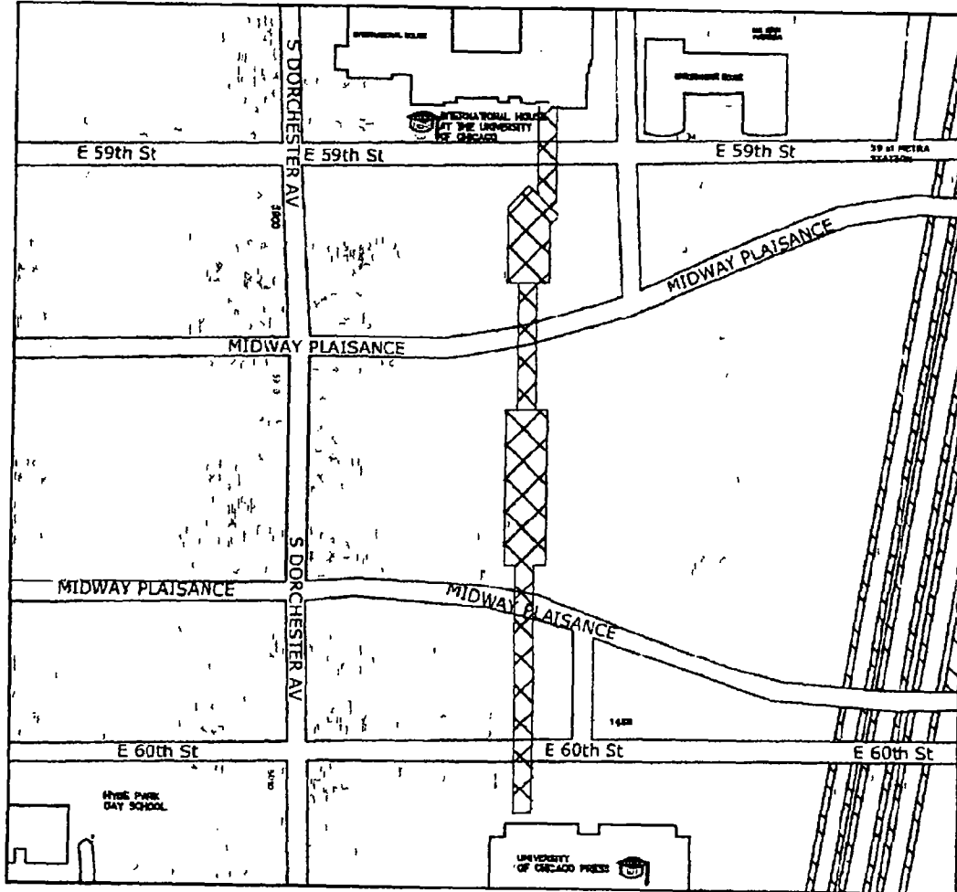
Chilled Water Lines at 59 th - 60 th /Dorchester University of Chicago
