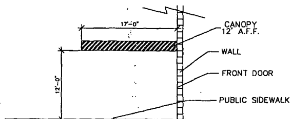
E.2 DOOR CANOPY SIDE VIEW SCALE: 1/8" = 1'-0"
