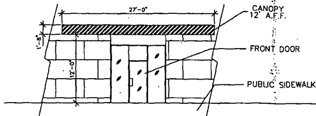
E.1 DOOR CANOPY FRONT VIEW SCALE: 1/8" = 1'-0"
