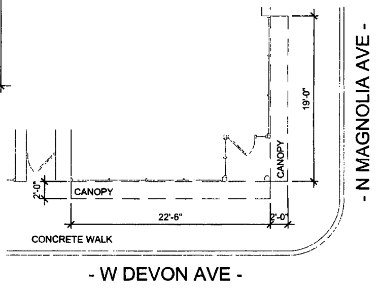
3 PLAN SCALE 1/8" = 1'-0"
