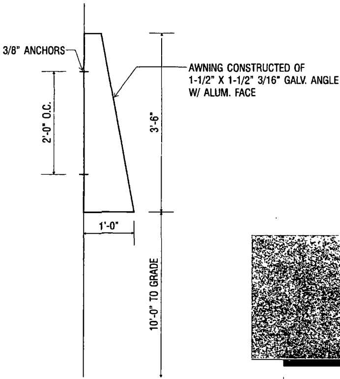
METAL AWNING - SIDE VIEW 3/4" = 1'-0"
