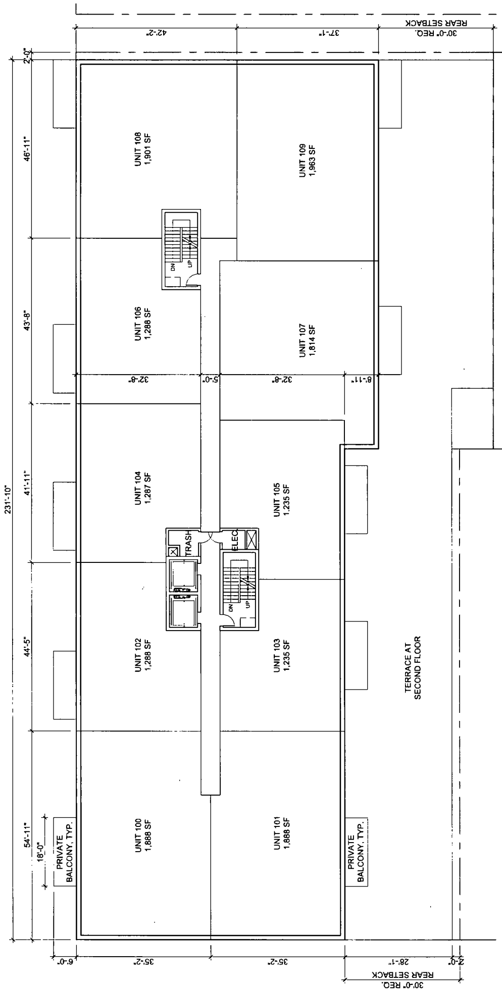
TYPICAL FLOOR PLAN FLOORS 2 - 6
