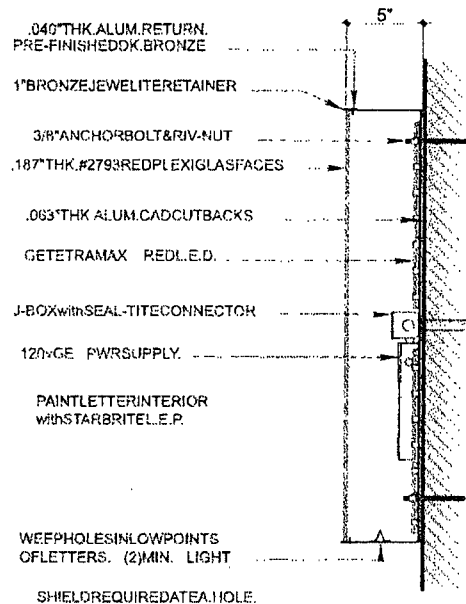
L.E.D. LETTERSECTION
