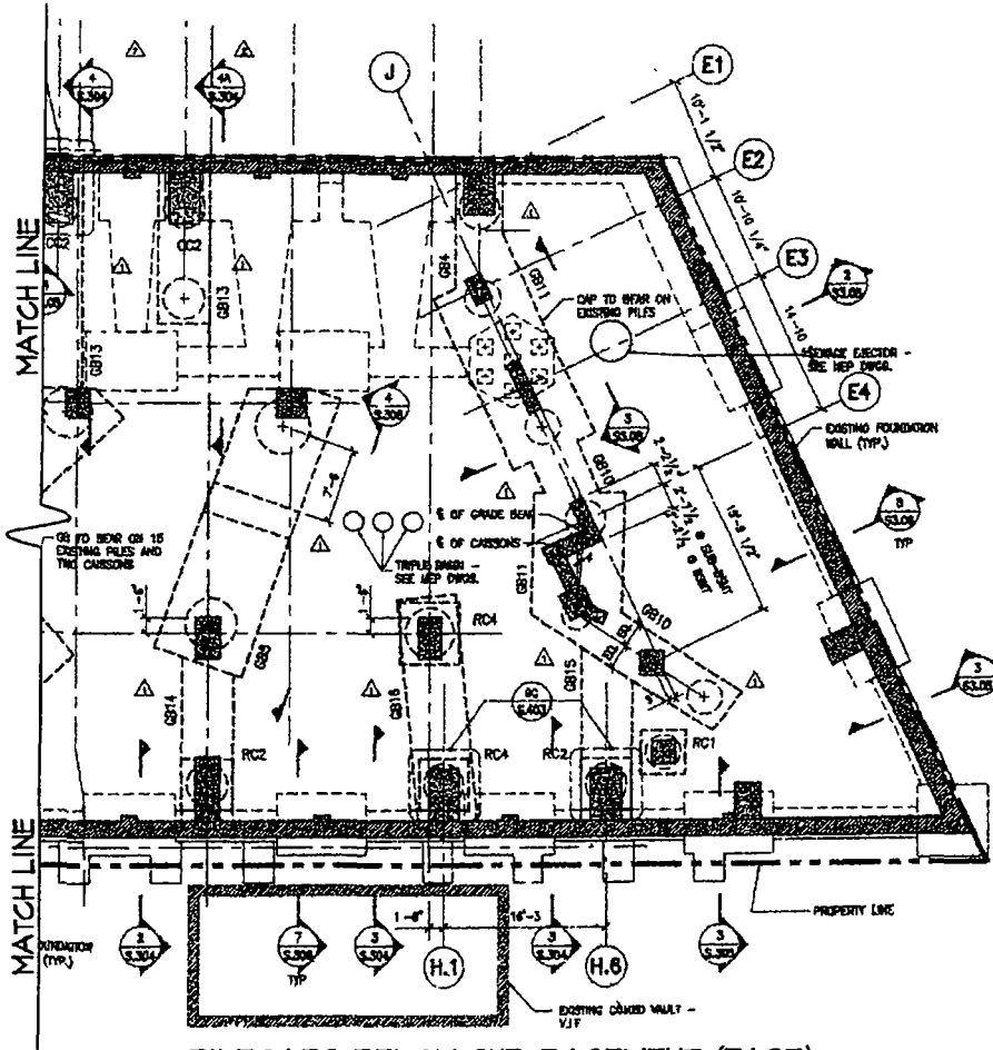
B PILECAPS BELOW SUB-BASEMENT (EAST) SCALE: 1/16" = 1'-0"
