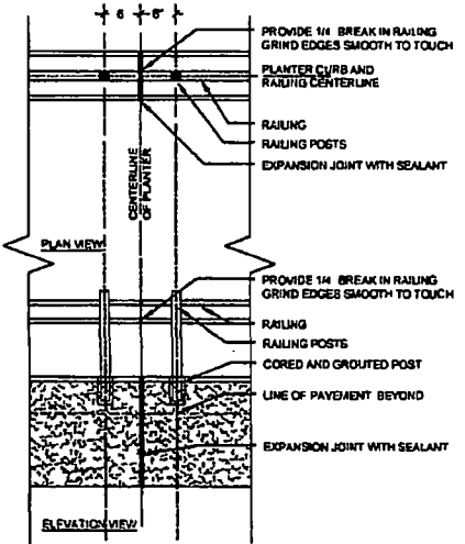
PLANTER CURB AND RAILING - MID-PLANTER DETAIL
