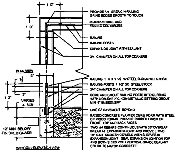
PLANTER CURB AND RAILING - CORNER DETAIL
