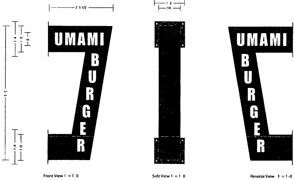
Front View 1 = 1 0
