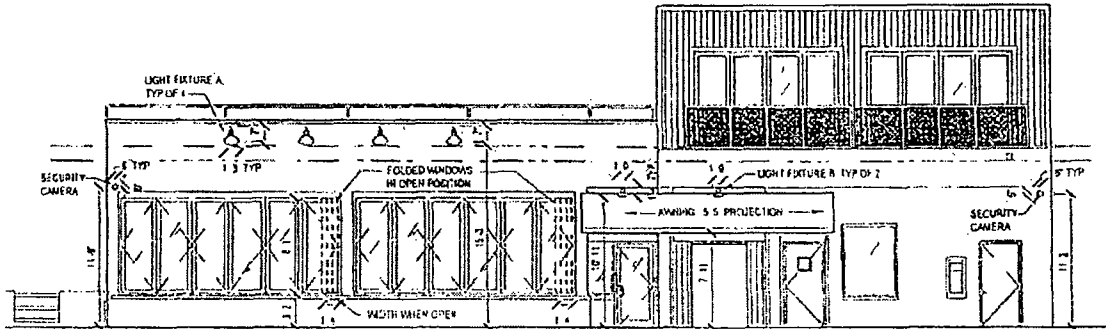
1 FRONT ELEVATION BUILDING & ENTRY SCALE 3/32" = 1'-0"
