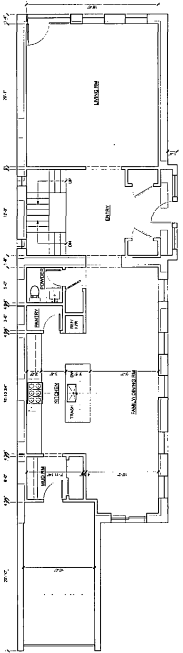
2 FIRST FLOOR PLAN Scale: 1/4" = 1'-0"
