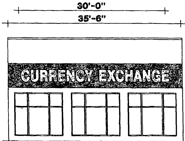
SOUTH ELEVATION
