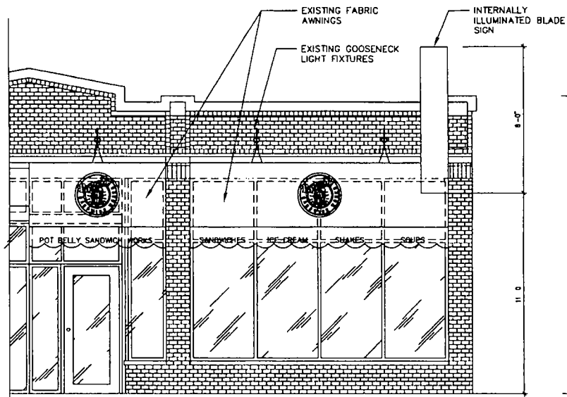
EXTERIOR ELEVATION
