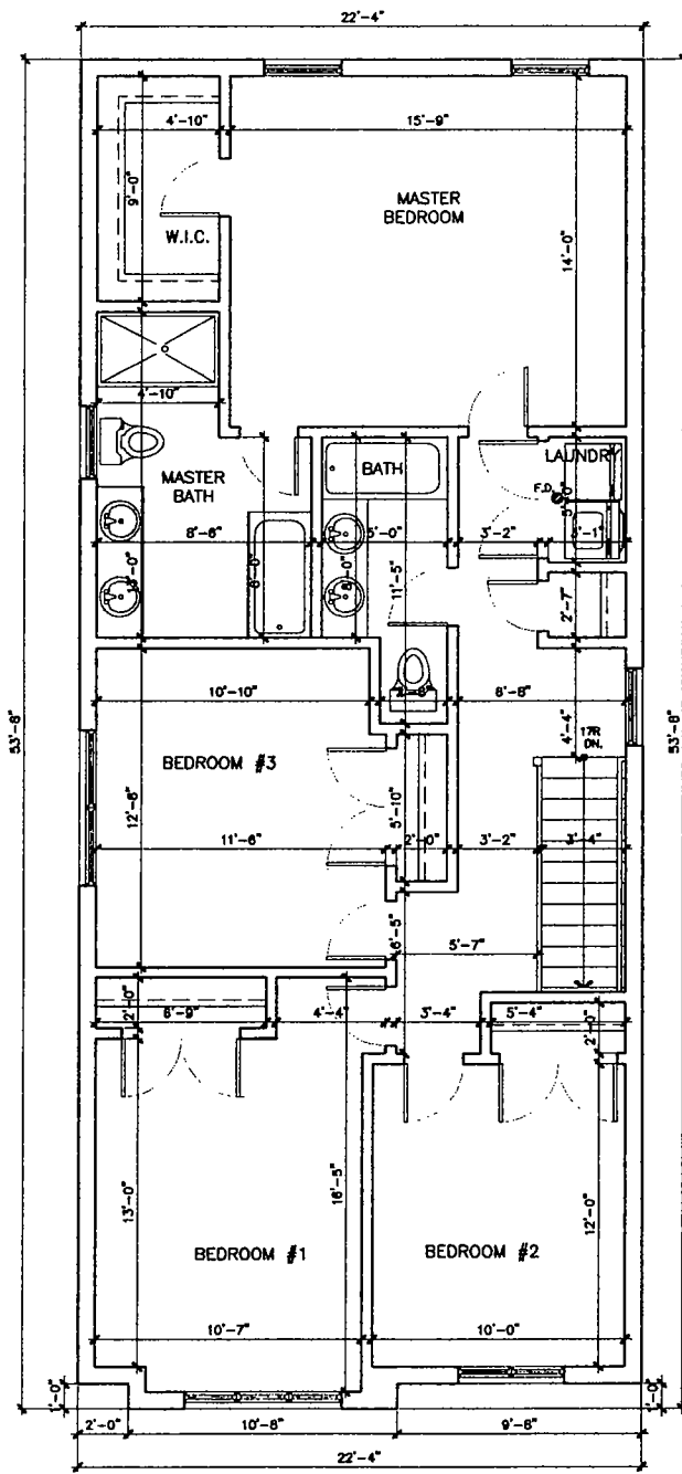
2ND. FLOOR PLAN SCALE: 3/16"=1'-0" 0 2' 4' 8'
