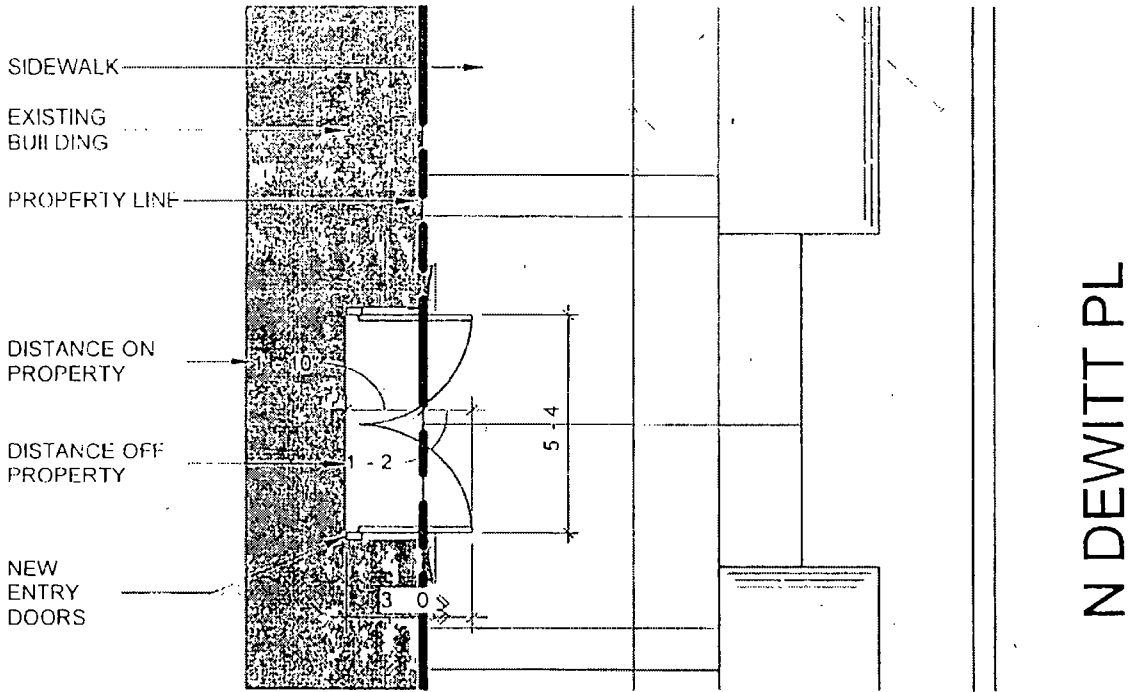
1 Site Plan-East Entry 1/4" = 1'-0"
