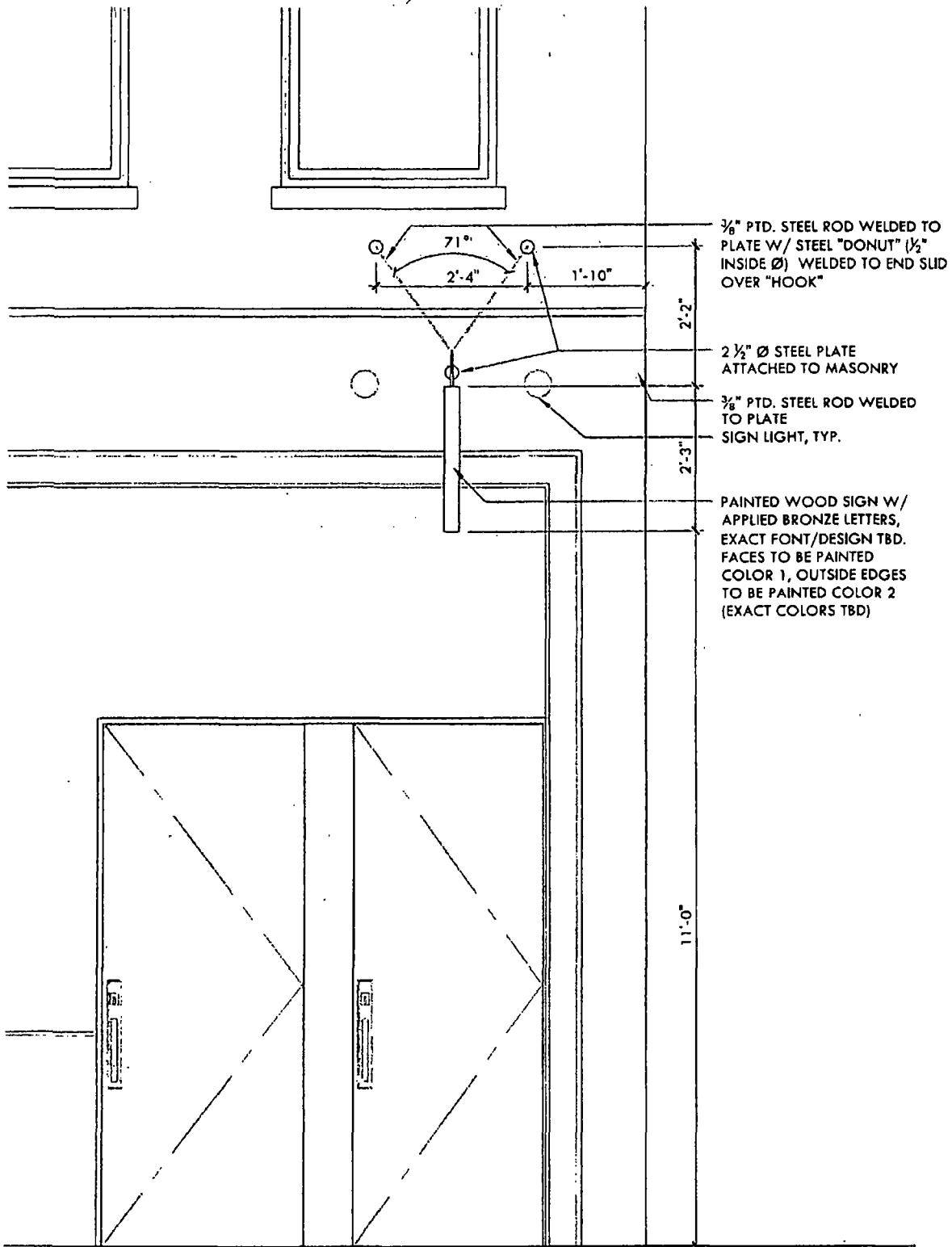
3 PARTIAL CLARK STREET ELEVATION (NORTH END OF BUILDING)
