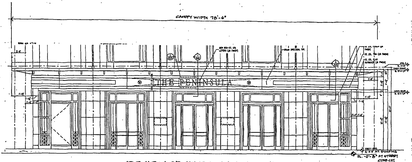
ELEVATION OF CANOPY AT SUPERIOR STREET.
