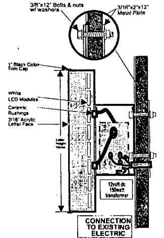
CHANNEL LETTER DETAIL NOT SCALE
