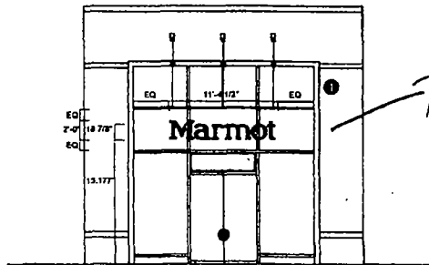
Front V. low SCALE: 1/8" = 1'-0"
