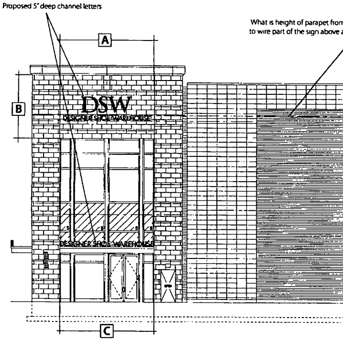
East Elevation
