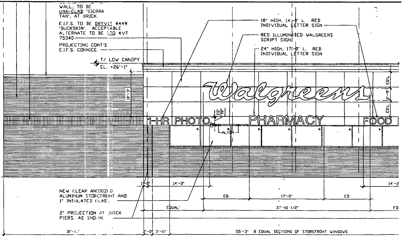
SOUTH ELEVATION (W. FULLERTON AVENUE) SCALE: 1/8" = 1'-0"
