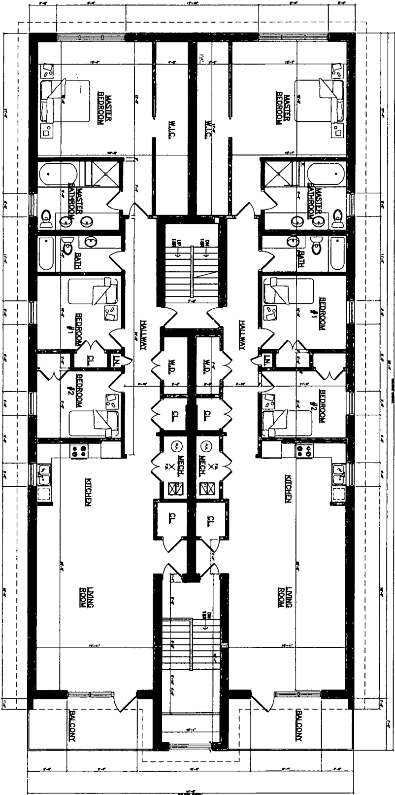
FOURTH FLOOR PLAN SCALE: 1/8" = 1'-0"
