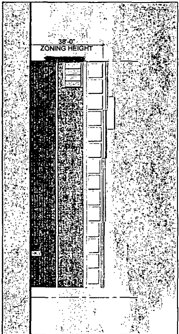
WEST ELEVATION
