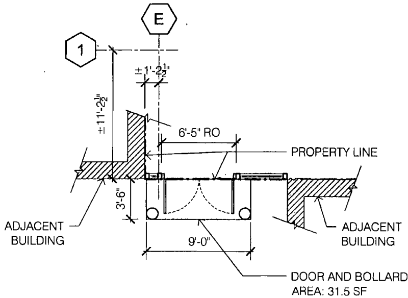
1 PARTIAL PLAN
