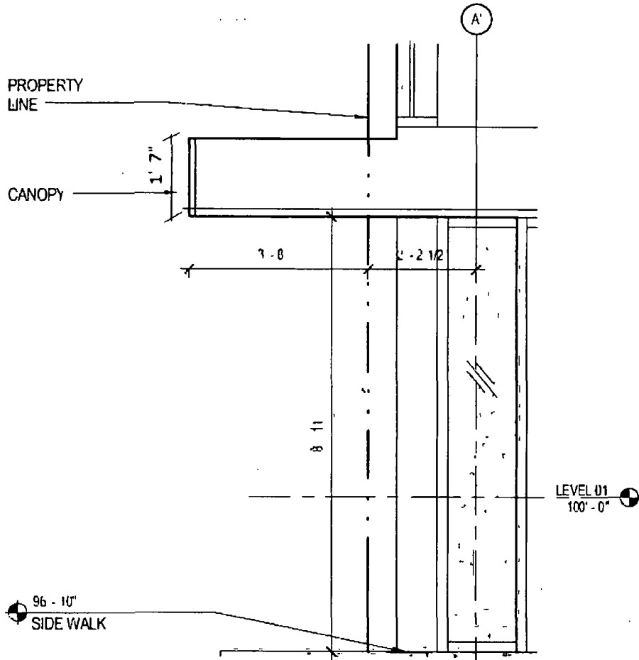
1 CANOPY SECTION PW 03 1/2 = 1 0
