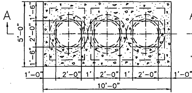
PLAN AND SECTION C-C
